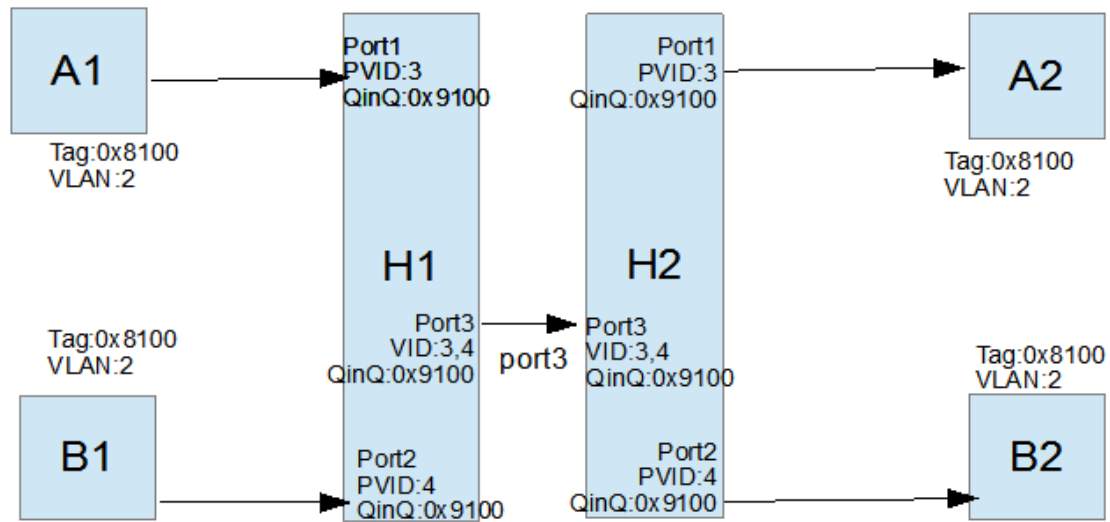
Figure 2.143 Example of QinQ Deployment
