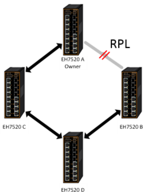
Figure 2.168 An Example of Ring Topology (Example made on EH7520)
