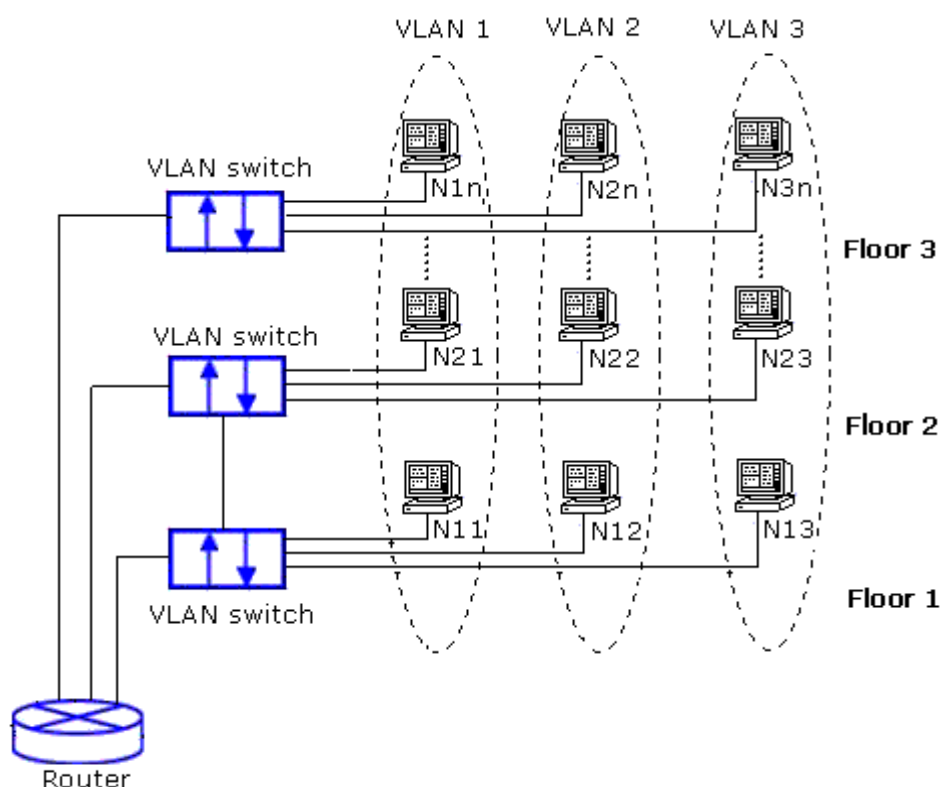
Figure 2.130 Example of VLAN Configuration
