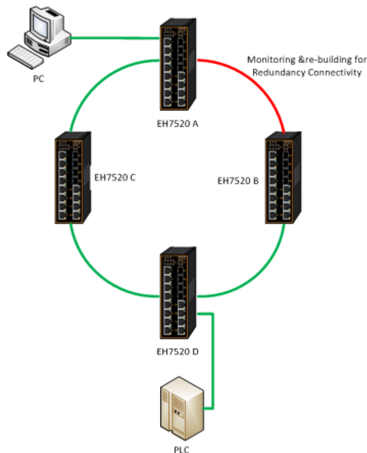
Figure 2.177 iA-Ring Example Topology (Example made on EH7520)
