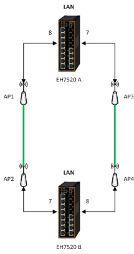
Figure 2.181 Example 2 of Two Wired Bridge U-ring (Example on EH7520)
