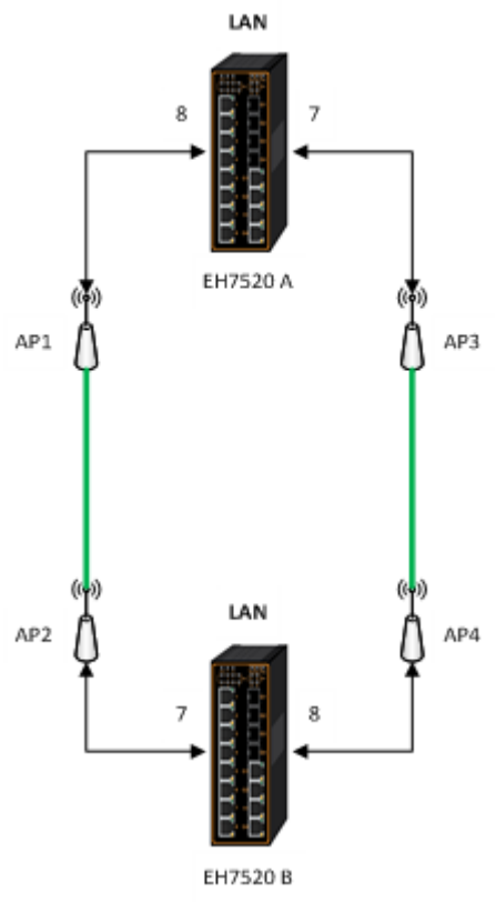
Figure 2.181 Example 2 of Two Wired Bridge U-ring (Example on EH7520)
