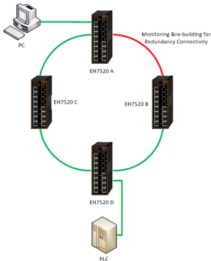
Figure 2.137 iA-Ring Example Topology (Example made on EH7520)
