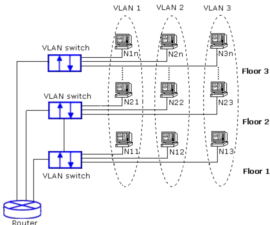
Figure 2.104 Example of VLAN Configuration
