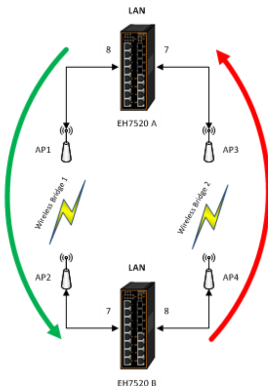
Figure 2.140 Example 1 of Two Wireless Bridge U-ring (Example made on EH7520)
