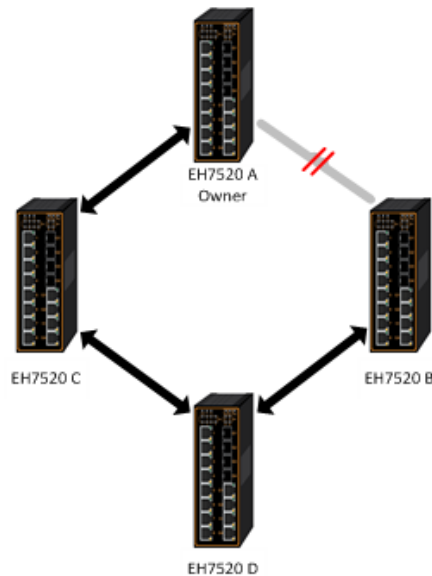
Figure 2.195 Example of Ring Topology for ERPS Setup (Example made on EH7520)
