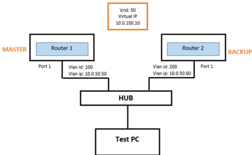
Figure 2.163 Overview of the VRRP
