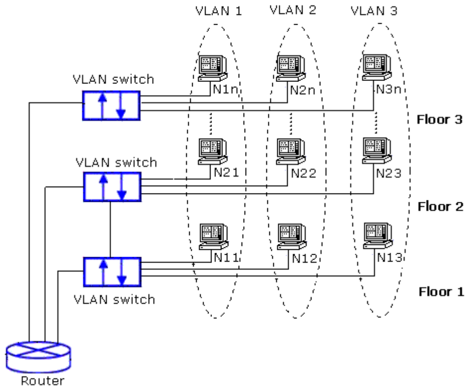
Figure 2.148 Example of VLAN Configuration
