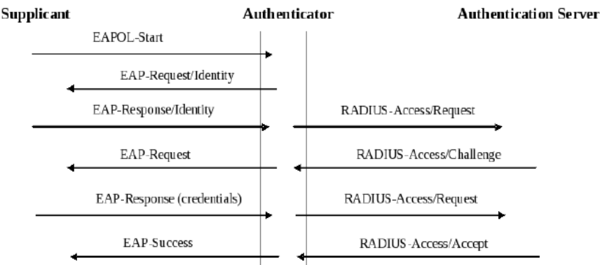
Figure 2.183 RADIUS Authentication Sequence
