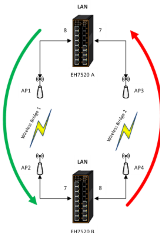
Figure 2.203 Example 1 of Two Wireless Bridge U-ring (Example made on EH7520)
