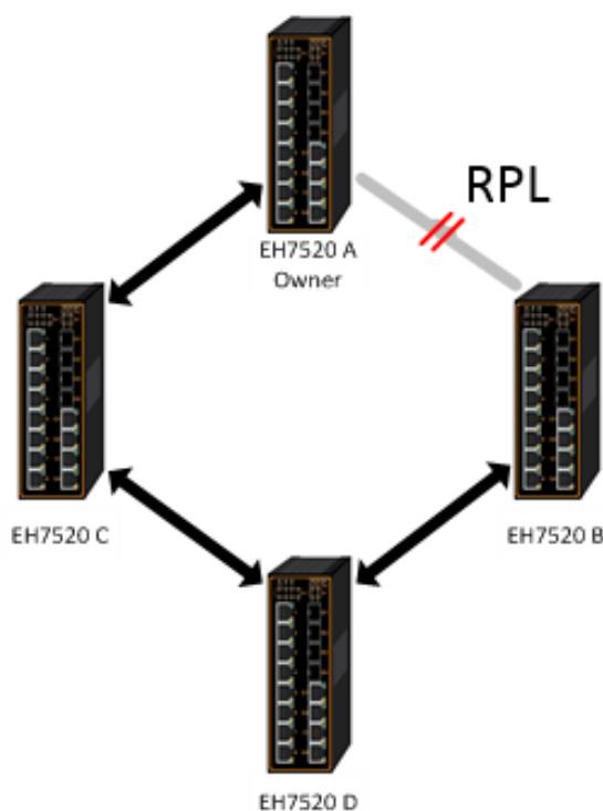
Figure 2.191 An Example of Ring Topology (Example made on EH7520)
