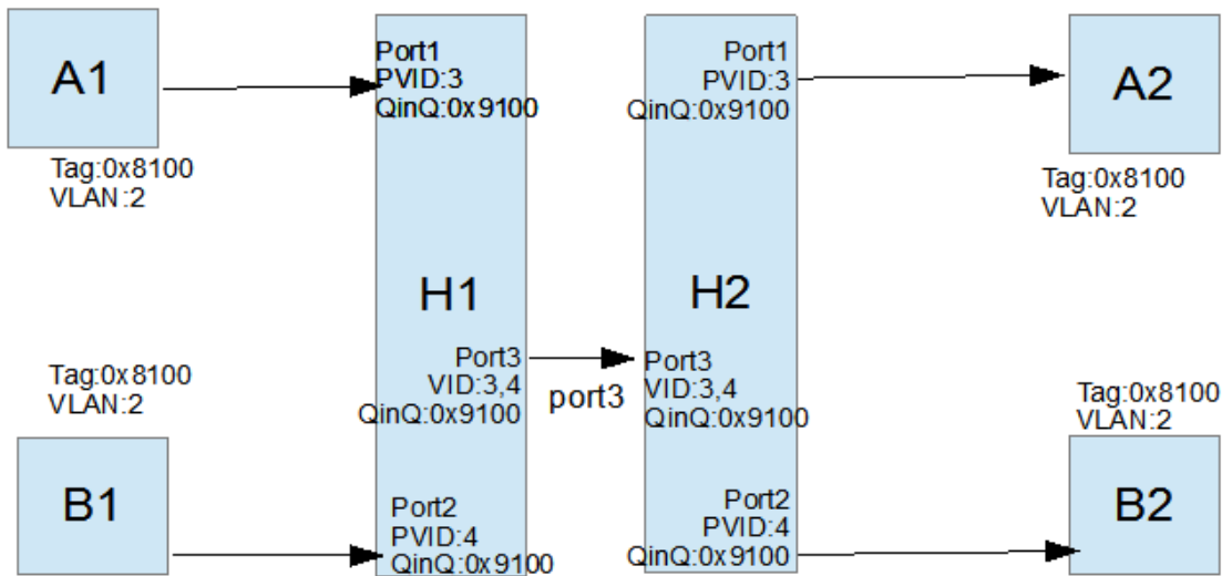
Figure 2.161 Example of QinQ Deployment
