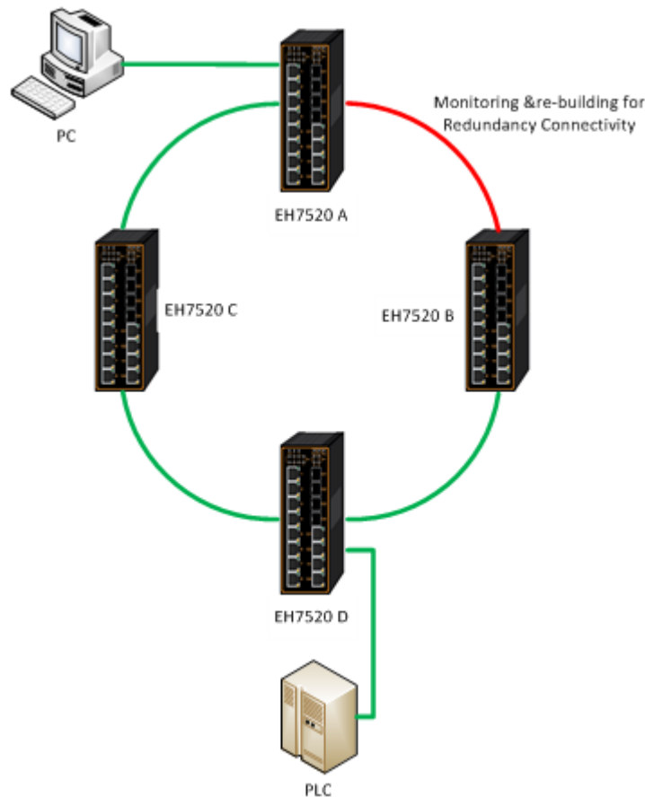
Figure 2.200 iA-Ring Example Topology (Example made on EH7520)
