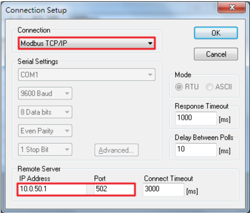
Figure 2.36 Modbus Poll Connection Setup
