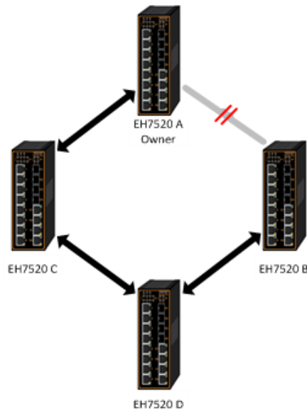
Figure 2.145 Example of Ring Topology for ERPS Setup (Example made on EH7520)
