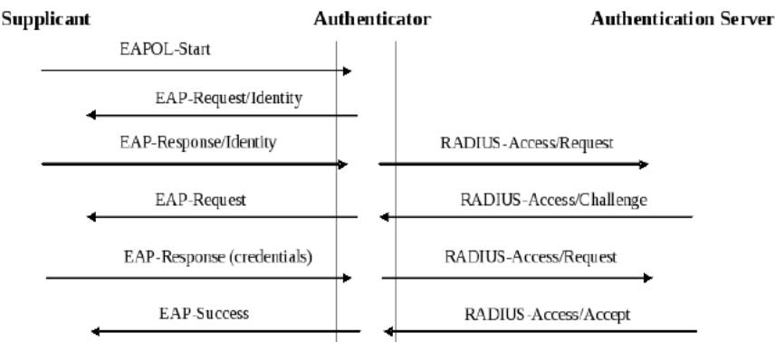
Figure 2.125 RADIUS Authentication Sequence
