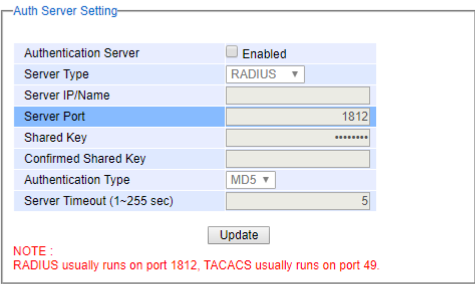
Figure 2.21 Authentication Server Setting
