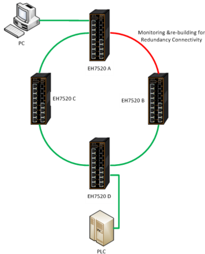
Figure 2.150 iA-Ring Example Topology (Example made on EH7520)
