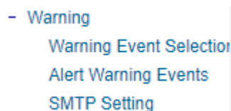
Figure 2.180 Warning Menu
