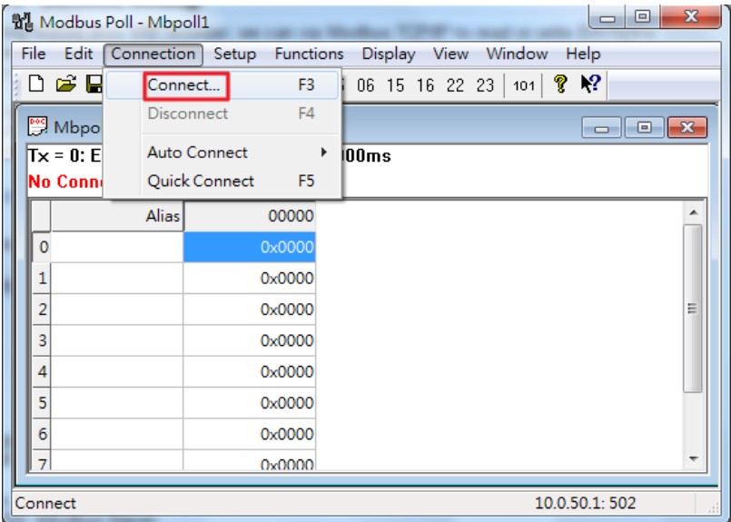
Figure 2.35 Entering Connection Setup Menu of the Modbus Poll
