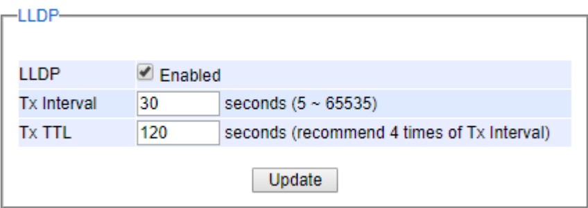
Figure 2.162 LLDP Setting Webpage
