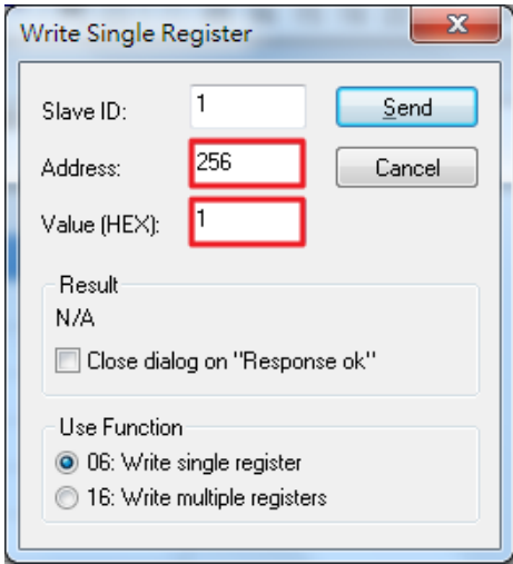
Figure 2.47 Use Modbus Poll to Clear Switch's Port Count
