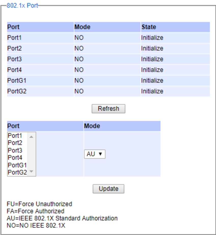
Figure 2.128 802.1x Port Setting Webpage
