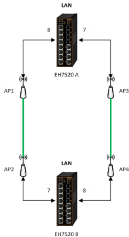
Figure 2.154 Example 2 of Two Wired Bridge U-ring (Example on EH7520)
