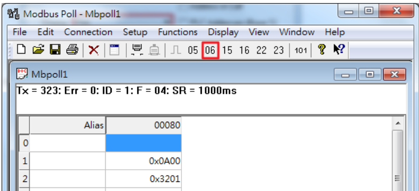
Figure 2.46 Click on Function 06 in the Modbus Poll
