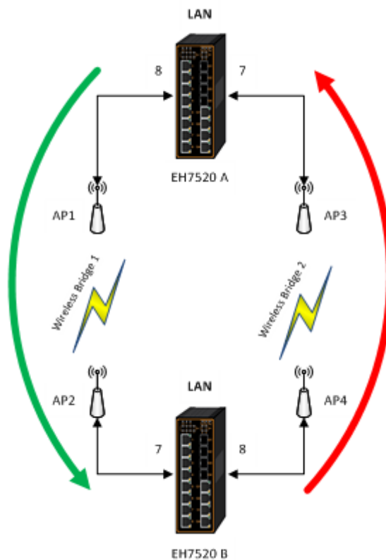
Figure 2.153 Example 1 of Two Wireless Bridge U-ring (Example made on EH7520)
