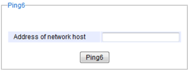
Figure 2.29 Ping6 Webpage
