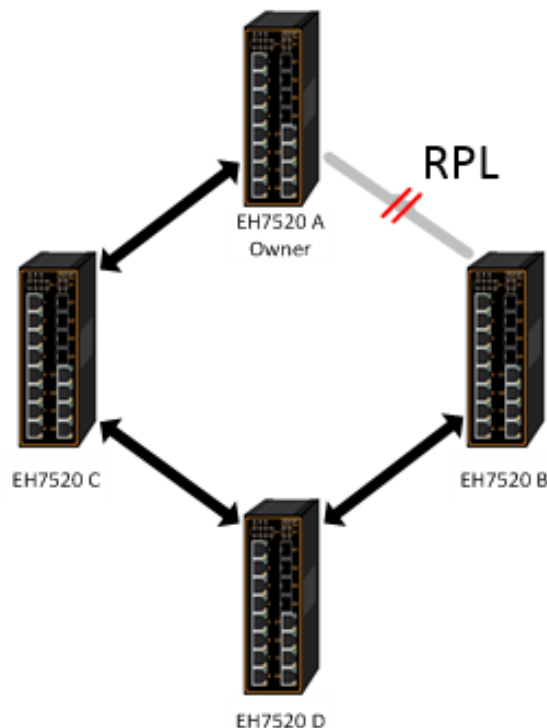
Figure 2.141 An Example of Ring Topology (Example made on EH7520)
