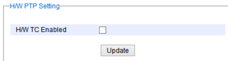
Figure 2.55 Hardware PTP Setting
