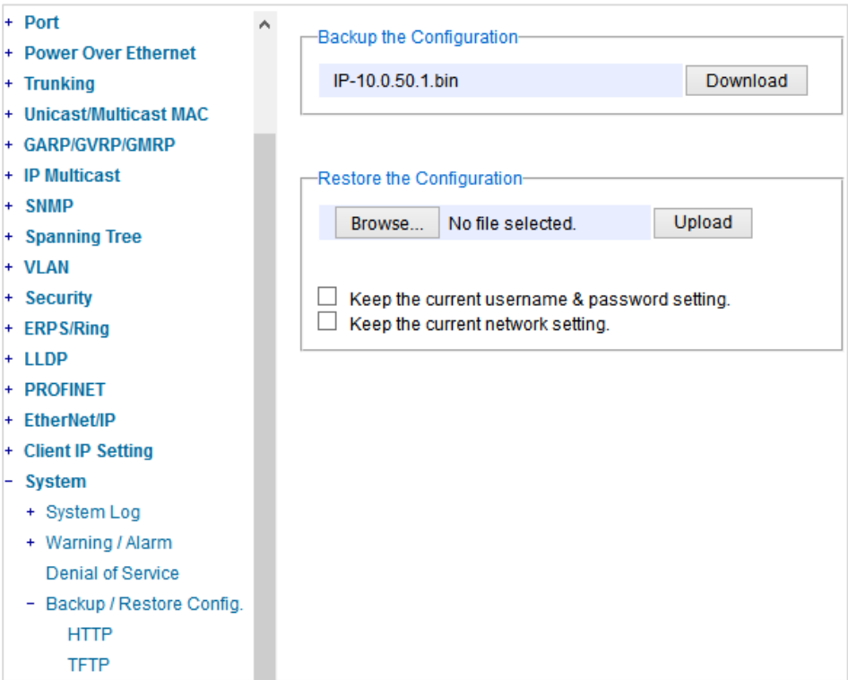
Figure 2.192 Backup/Restore Config. Dropdown Menu
