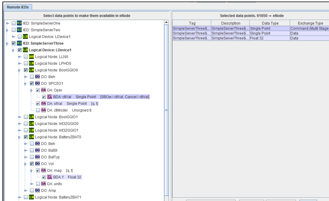
Figure 2-2 - Main screen.
