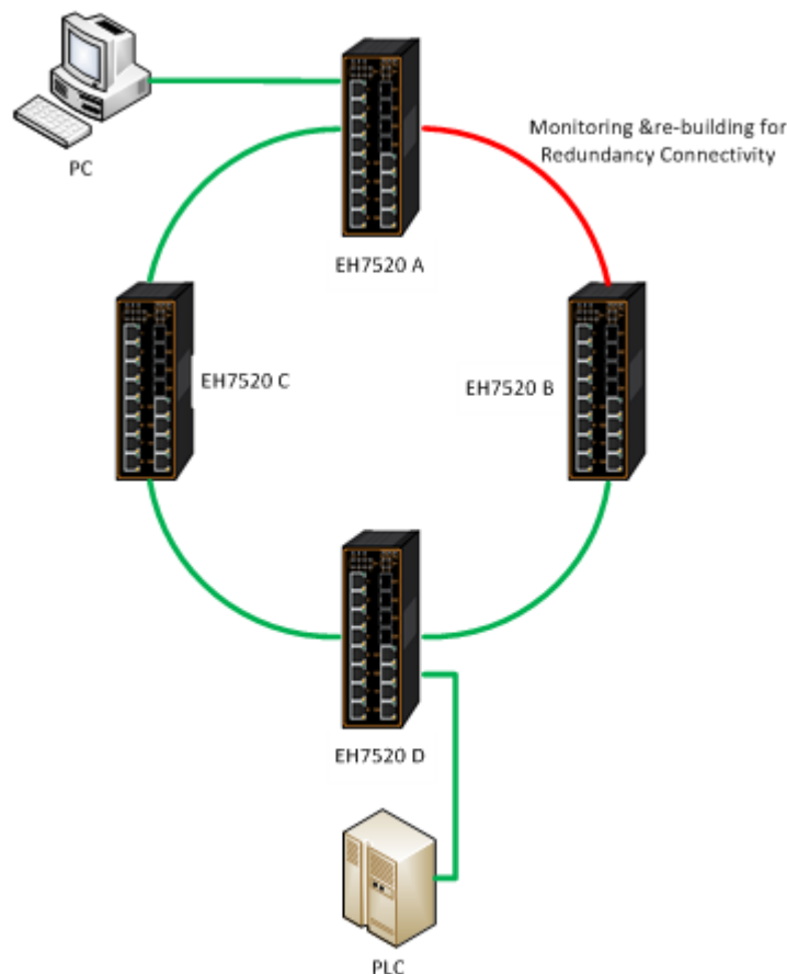
Figure 2.152 iA-Ring Example Topology (Example made on EH7520)
