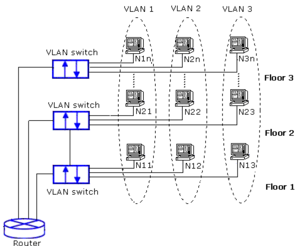
Figure 2.109 Example of VLAN Configuration
