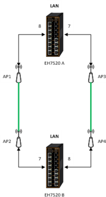
Figure 2.156 Example 2 of Two Wired Bridge U-ring (Example on EH7520)
