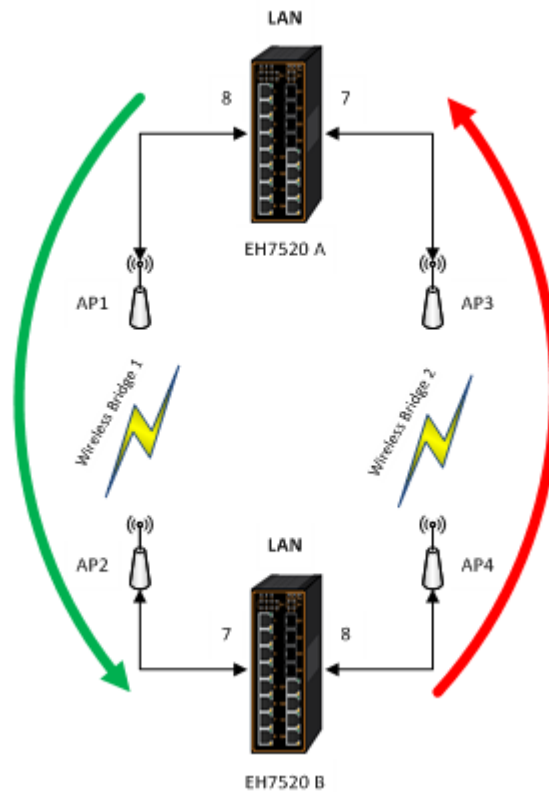
Figure 2.155 Example 1 of Two Wireless Bridge U-ring (Example made on EH7520)
