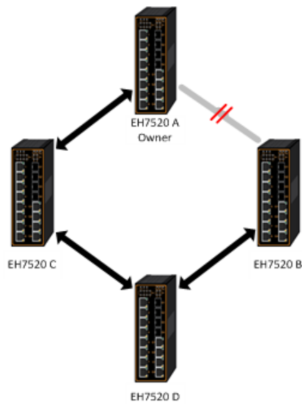
Figure 2.147 Example of Ring Topology for ERPS Setup (Example made on EH7520)
