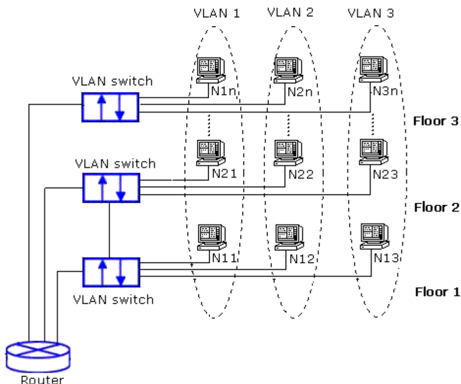
Figure 2.146 Example of VLAN Configuration
