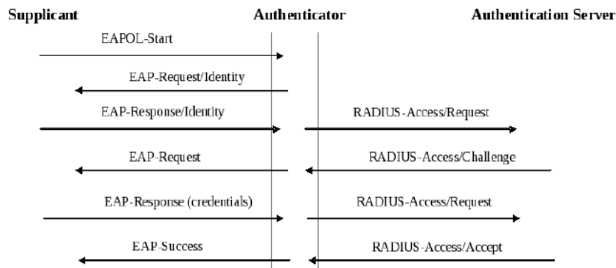
Figure 2.181 RADIUS Authentication Sequence
