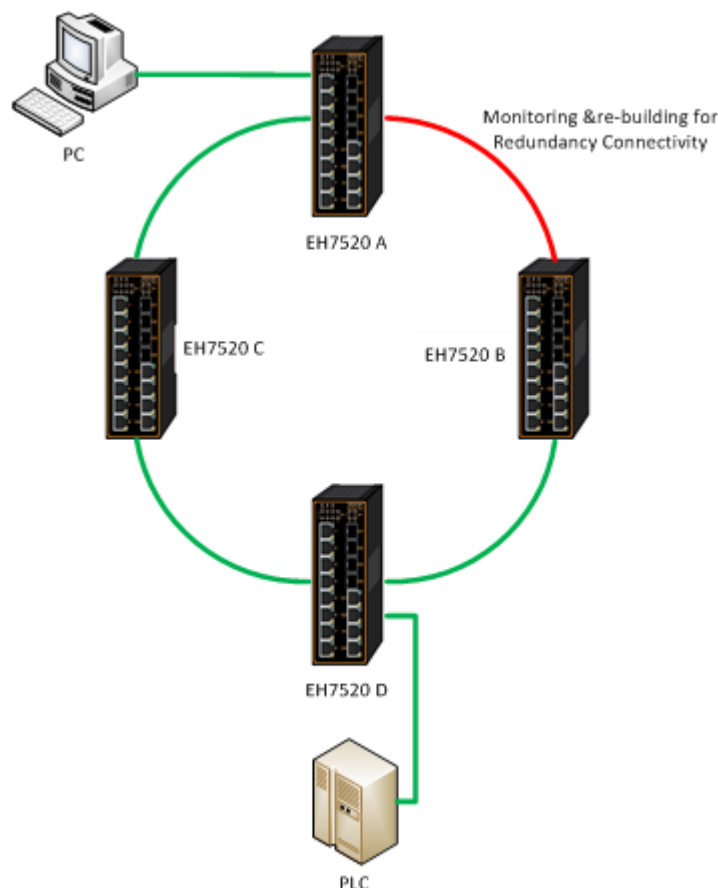
Figure 2.198 iA-Ring Example Topology (Example made on EH7520)
