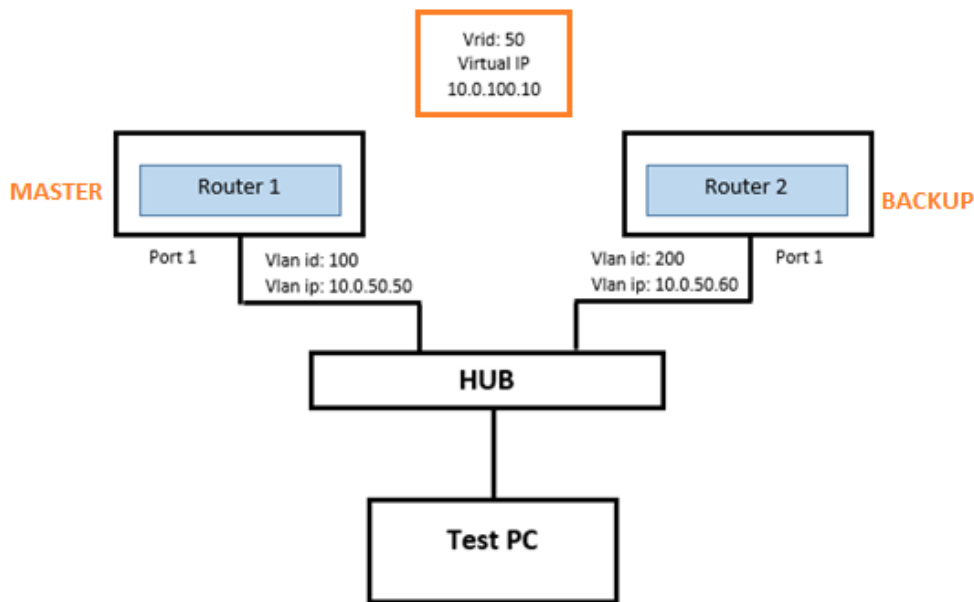
Figure 2.161 Overview of the VRRP
