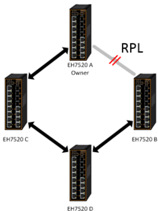
Figure 2.189 An Example of Ring Topology (Example made on EH7520)
