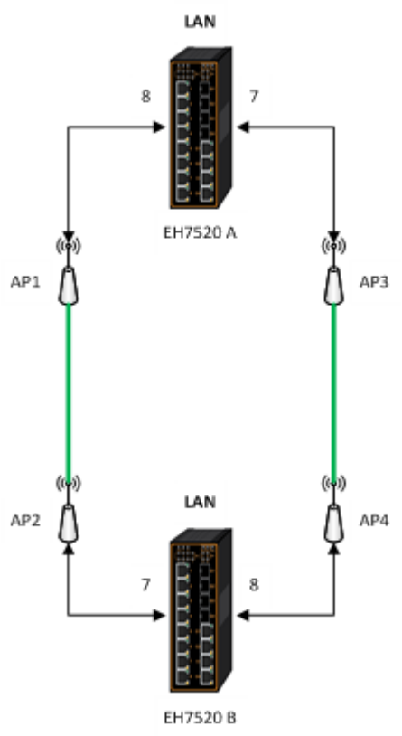
Figure 2.202 Example 2 of Two Wired Bridge U-ring (Example on EH7520)
