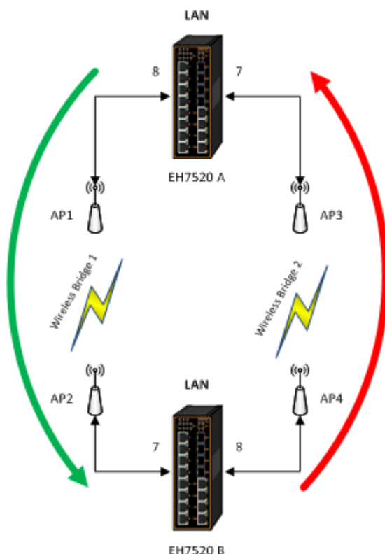
Figure 2.201 Example 1 of Two Wireless Bridge U-ring (Example made on EH7520)
