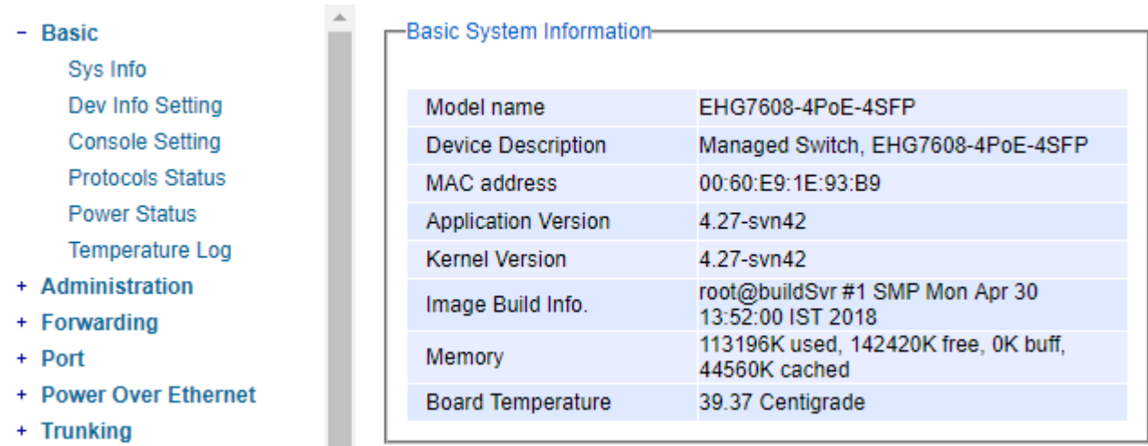
Figure 2.3 Basic Information Dropdown Menu
