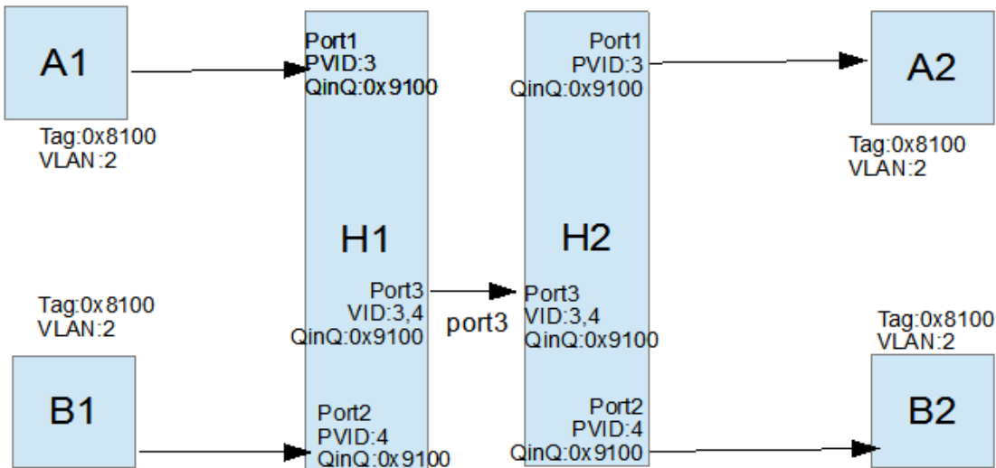
Figure 2.159 Example of QinQ Deployment
