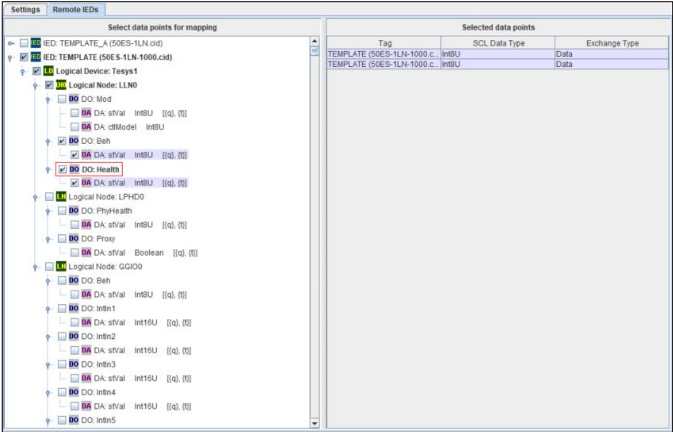
Figure 2-2 - Main screen.
