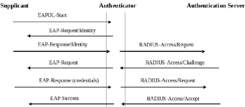
Figure 2.225RADIUS Authentication Sequence
