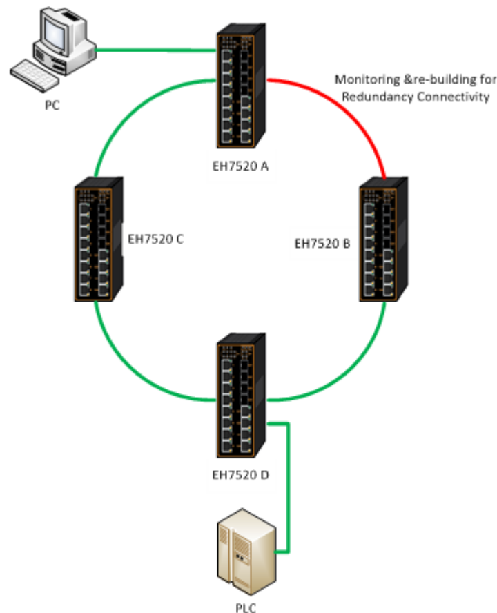
Figure 2.250iA-Ring Example Topology (Example made on EH7520)
