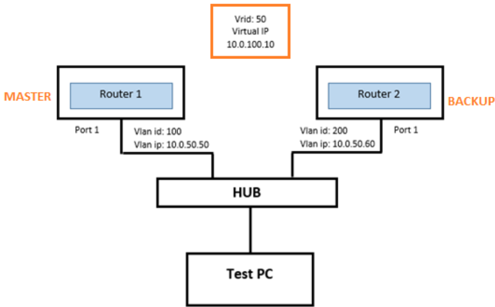
Figure 2.205 Overview of the VRRP
