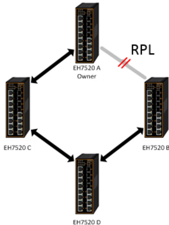
Figure 2.241 An Example of Ring Topology (Example made on EH7520)
