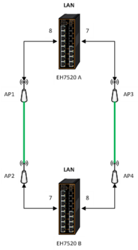
Figure 2.254 Example 2 of Two Wired Bridge U-ring (Example on EH7520)
