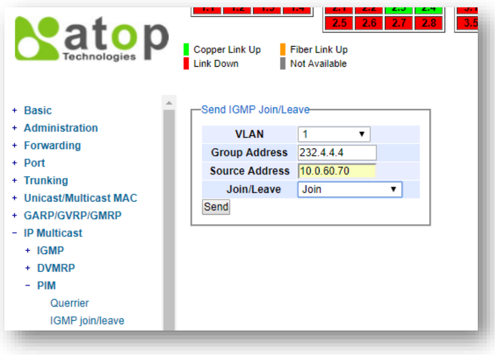
Figure 2.122 Example of Sending IGMP Join to an SSM Source Address
