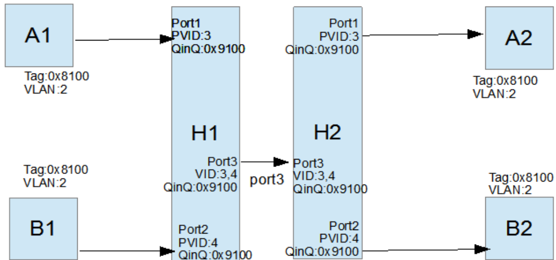
Figure 2.203 Example of QinQ Deployment
