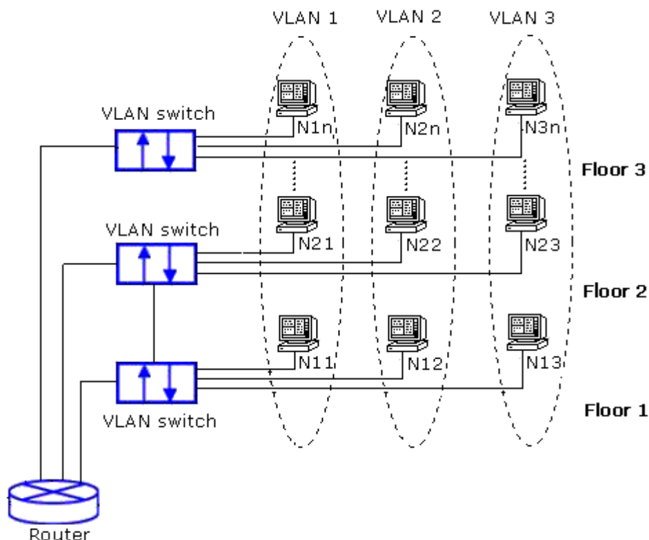
Figure 2.190Example of VLAN Configuration
