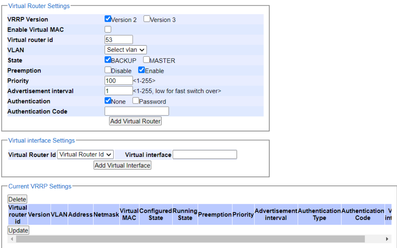
Figure 2.208Setting in VRRPMenu
