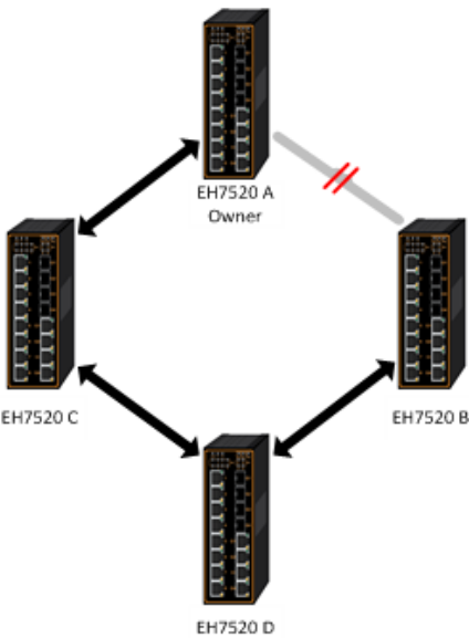
Figure 2.245Example of Ring Topology for ERPS Setup (Example made on EH7520)
